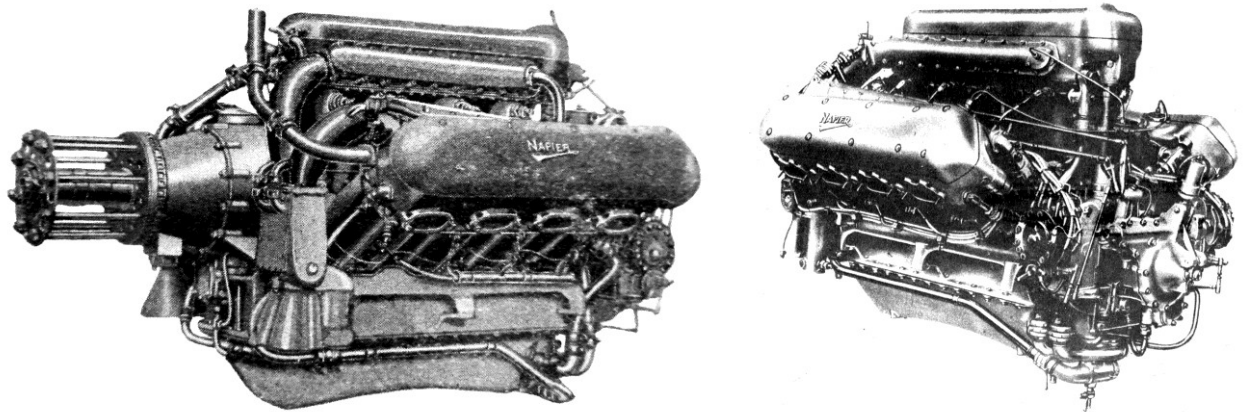
Motor Napier Lion 450 hp
